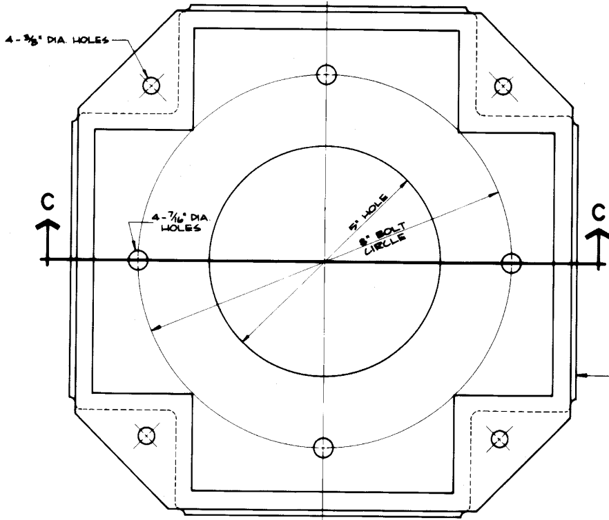
TERMINAL BOX INSIDE VIEW FROM TOP
